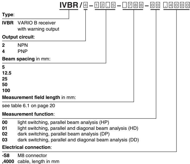
Figure 6.2: Type code VARIO B - receiver
